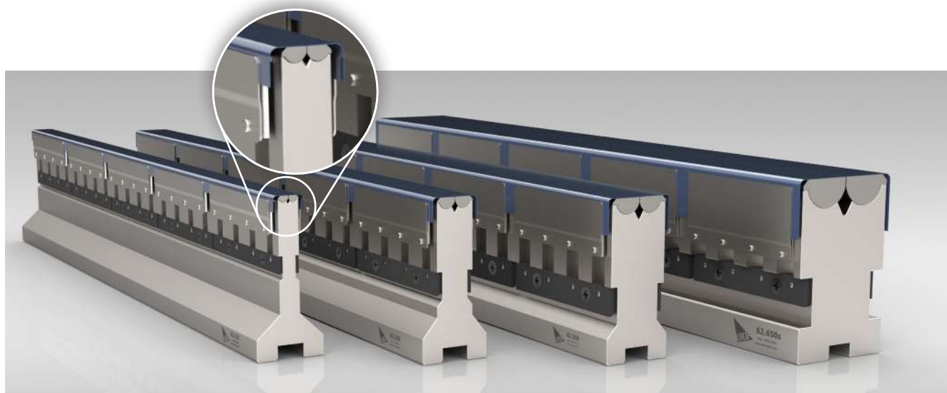
WingBend PLUS ondergereedschappen 62.120, 62.230, 62.350 en 62.650s (incl. Slider)
